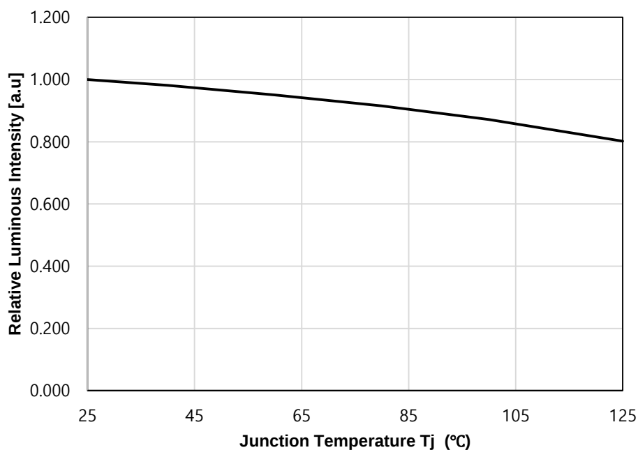
Fig 6. Junction Temperature vs. Relative Luminous Intensity, I_F=65\text{mA}
